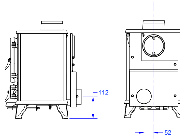
Direct air option inlet
