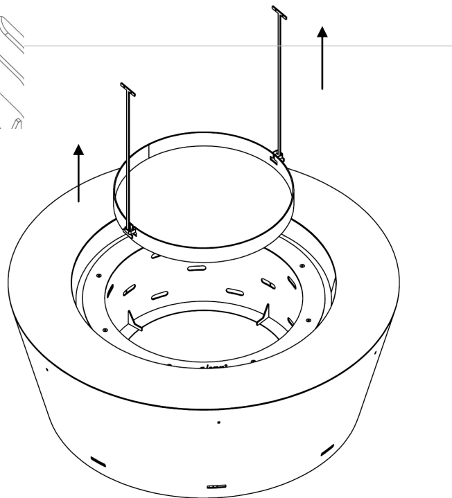
Figure 9 – Ashtray removal
