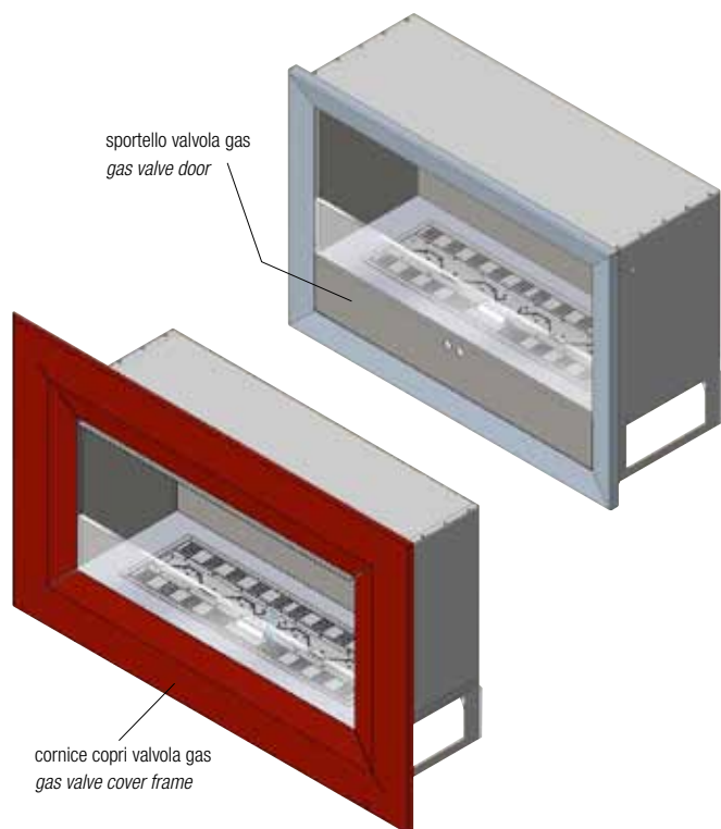
valvola remotata remote valve
