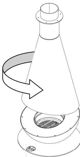
Figure 14 - Top rotation
