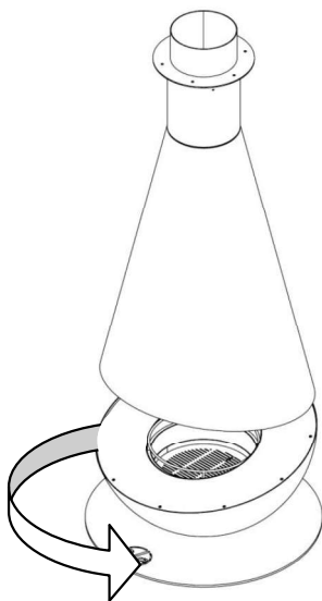
Figure 13 - Rotation of the lower part
