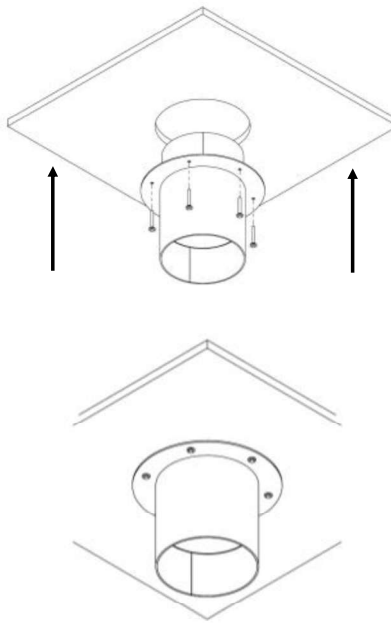
Figure 1 - Top part to screw to the ceiling
