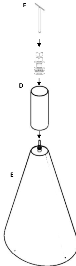
Figure 4- Representation of the assembly
